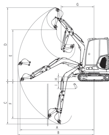
Working range schematic diagram
